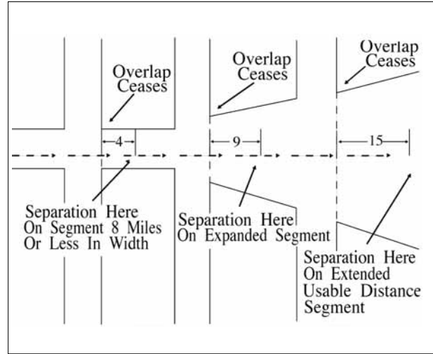
RNAV Minima
