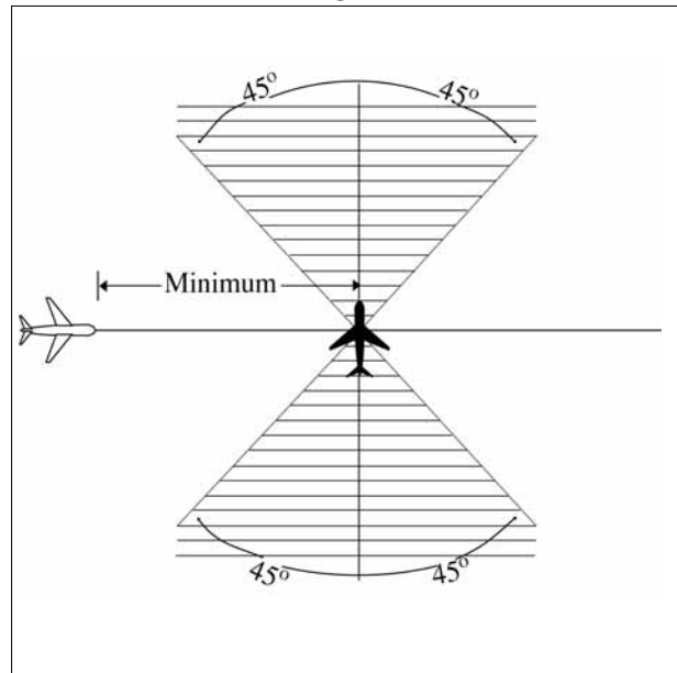
Crossing Courses
